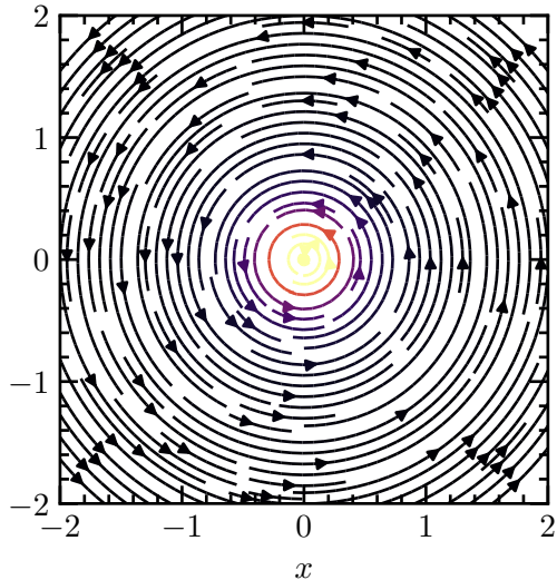
Positive curl
