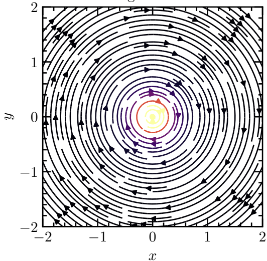
Negative curl
